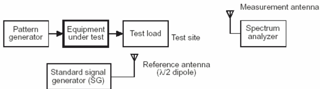
Figure 5.1.1.9: Measurement diagram for Cabinet radiation
