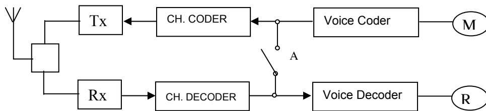
Figure 5.2 Measurement system diagram
