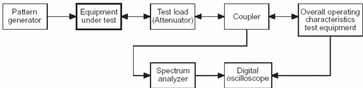
Figure 5.1.1.11b: Measurement system diagram b
