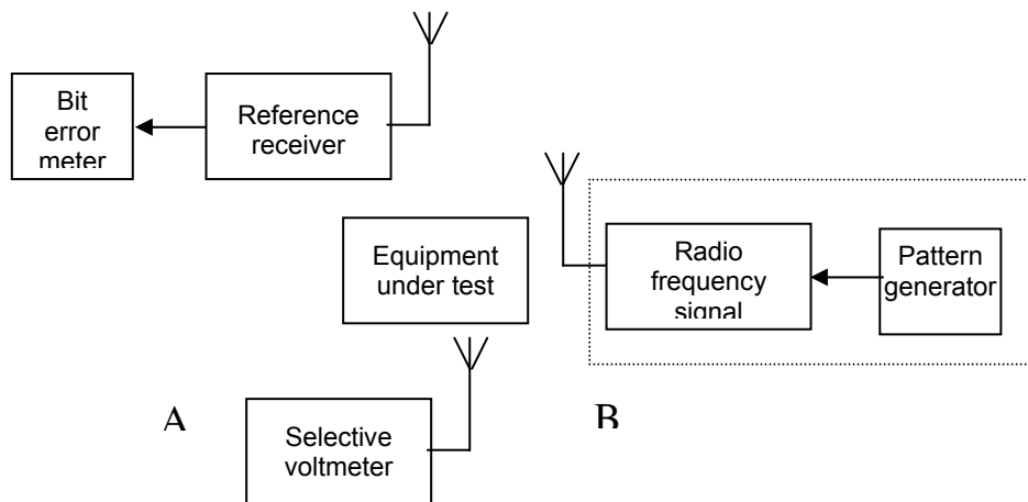
Figure 5.2.2.1.a: Measurement Diagram for Sensitivity (test site measurement)
