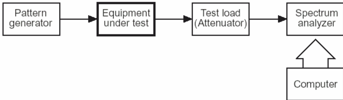
Figure 5.1.1.8: Measurement of Adjacent channel leakage power
