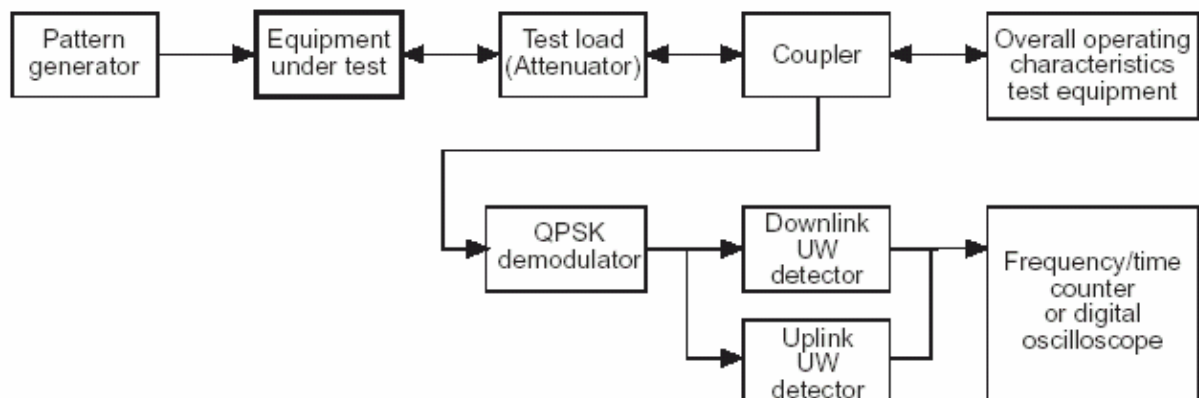
Figure 5.1.1.11a: Measurement system diagram for Transmission timing a
