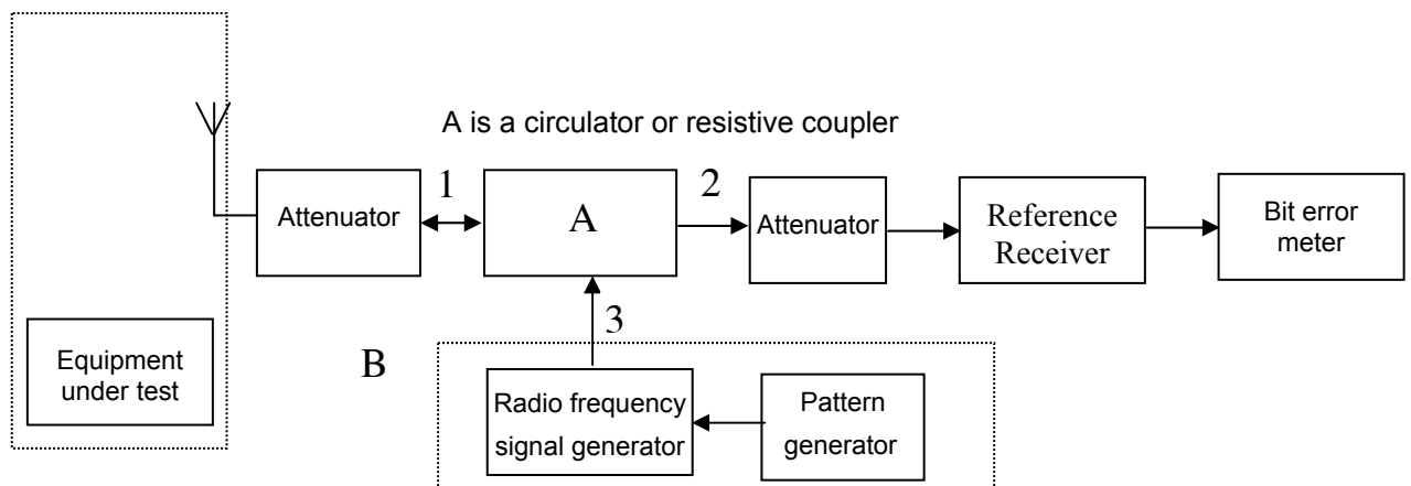
Figure 5.2.2.1.b: Measurement diagram when there is no data output terminal
