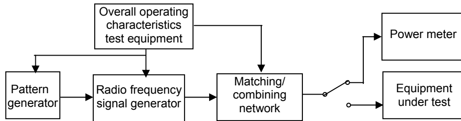
Figure 5.1.2.7: Measurement diagram for carrier sensing
