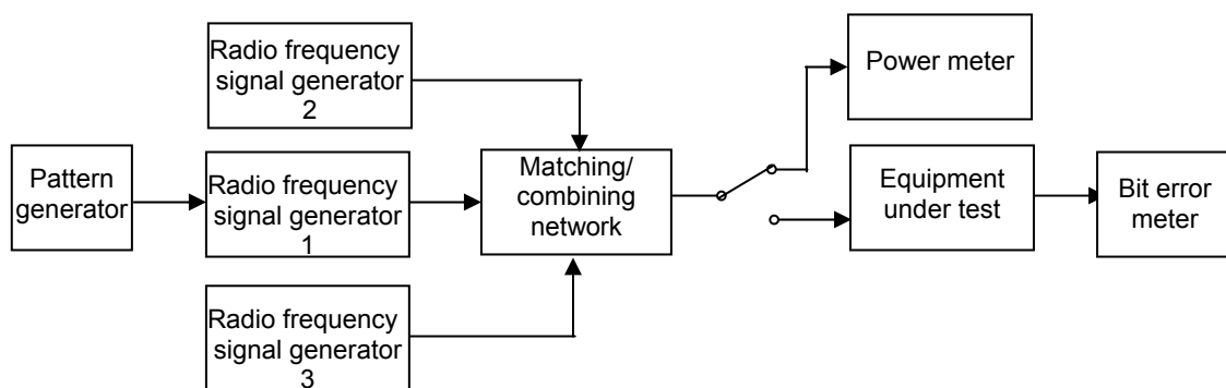
Figure 5.1.2.3 Measurement system diagram for Intermodulation characteristics
