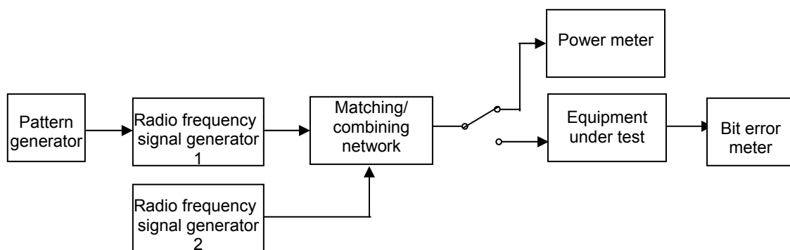
Figure 5.1.2.4 : Measurement system diagram for spurious response immunity
