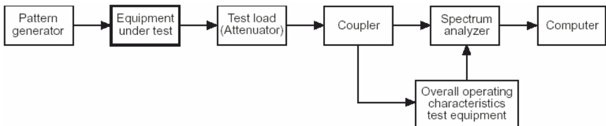
Figure 5.1.1.5: Measurement diagram of carrier offtime leakage power
