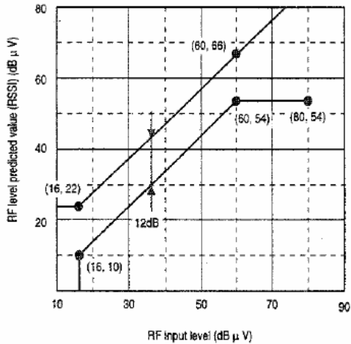
Figure 4.5: RF input level indicator accuracy
