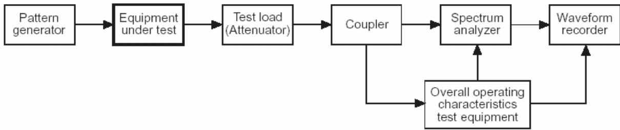
Figure 5.1.1.6 : Measurement diagram of transient characteristics of burst transmission
