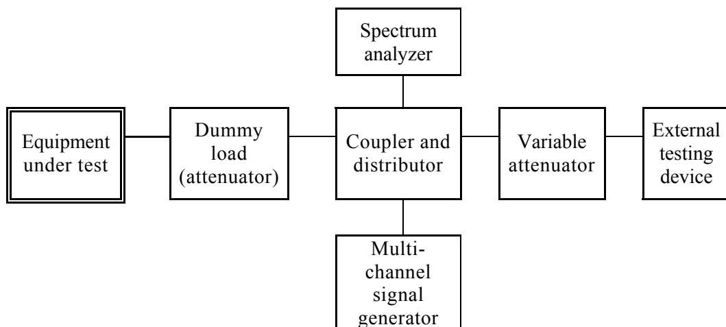
Figure 5.3.2 Measuring System Block Diagram for Control Channel
