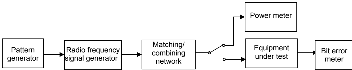
Fig 5.1.2.1 : Measurement system diagram for Sensitivity
