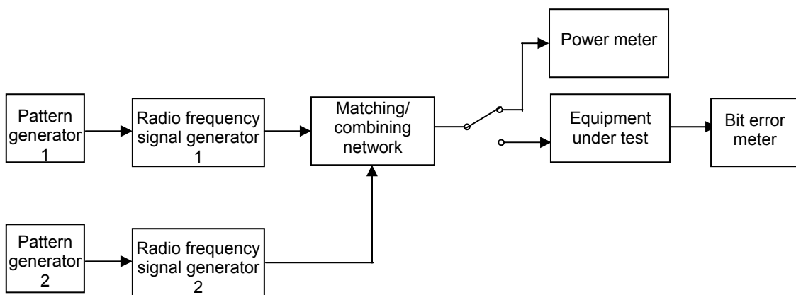
Figure 5.1.2.2: Measurement system diagram for Adjacent channel selectivity
