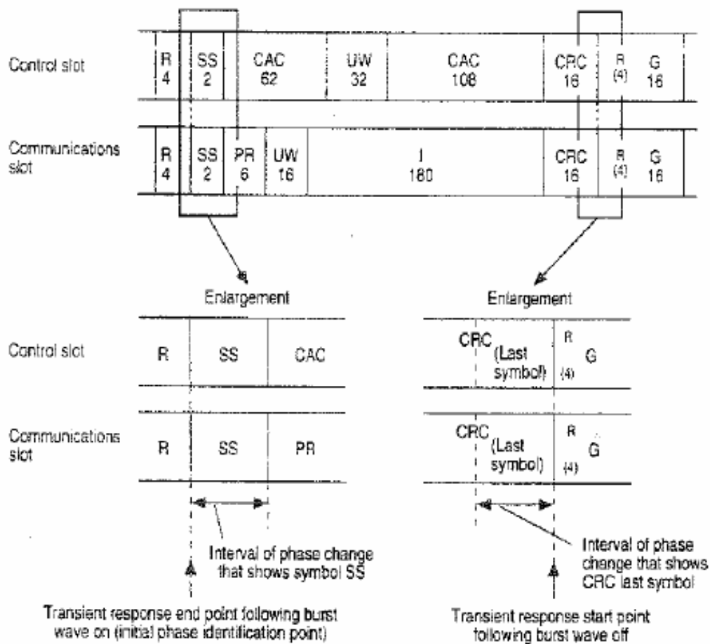
Figure 4.4 : Relationship between slot structure and burst wave on/off control
