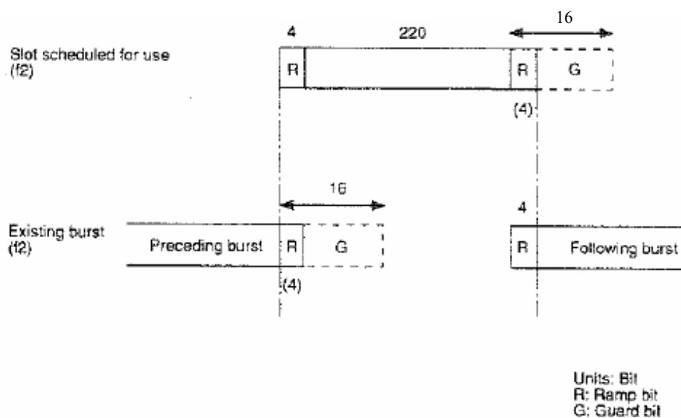
Figure 4.1: Carrier sensing method in PS side
