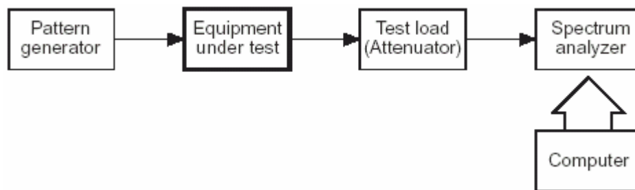
Figure 5.1.13 Measurement diagram of Occupied bandwidth
